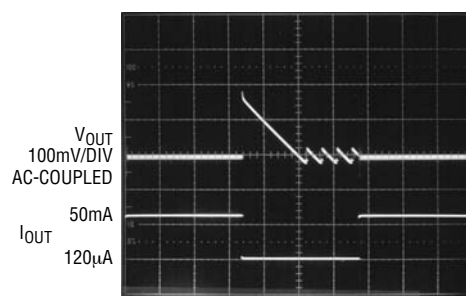
Fixed Frequency and Burst Mode Operation (LTC3429 Only)
