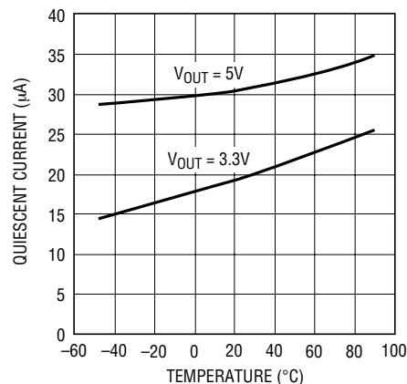
Burst Mode Quiescent Current vs Temperature (LTC3429 Only)
