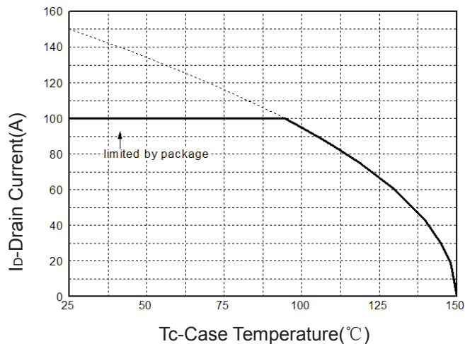
Figure 2: Drain Current
