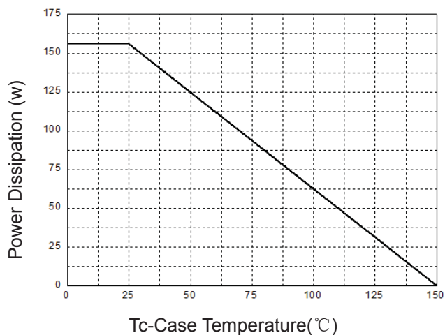
Figure 1: Power Dissipation
