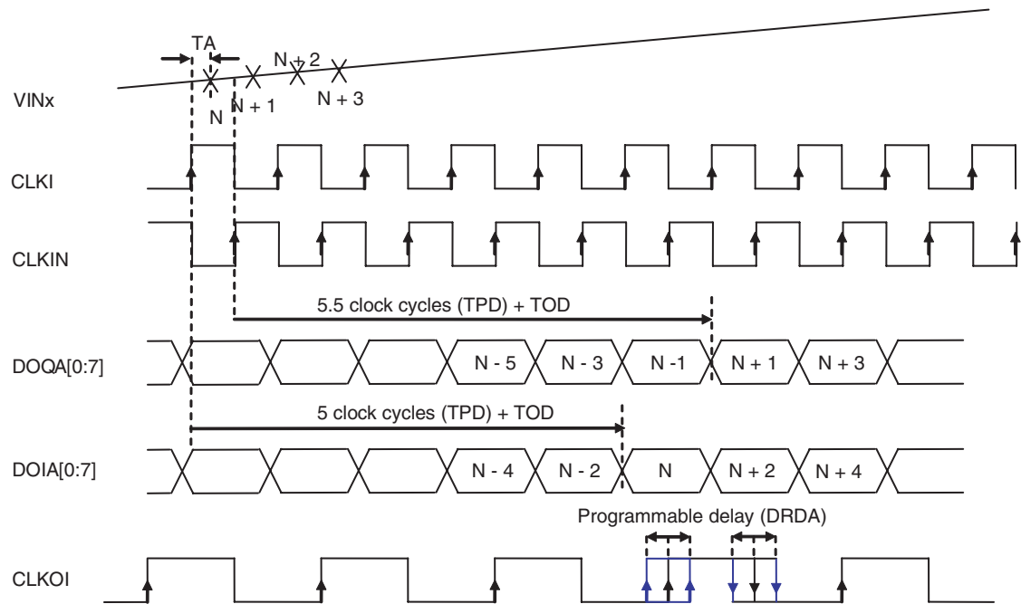
Figure 7-5. 1:1 DMUX Mode, Clock I → ADC I, Clock IN → ADC Q
