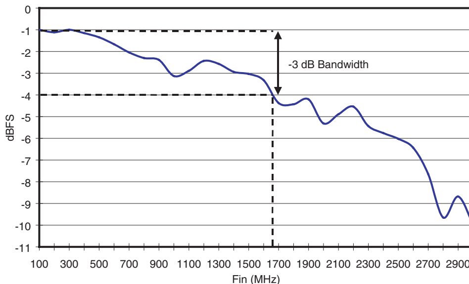
Figure 9-1. Full Power Input Bandwidth
