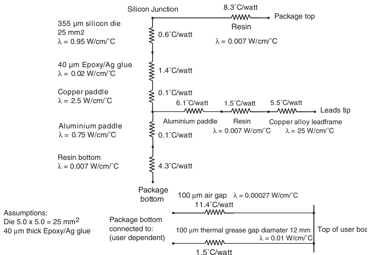
Figure 14-1. Simplified Thermal Model for LQFP Package
