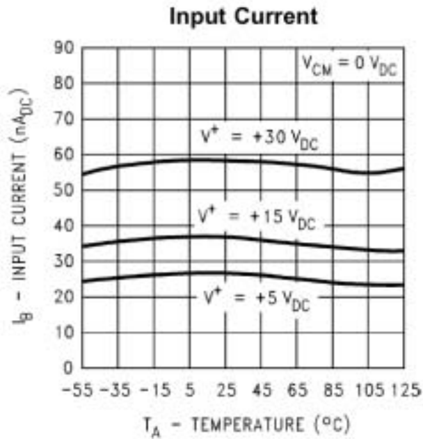
FIGURE 2. INPUT CURRENT
