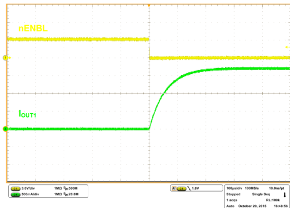
Figure 9. Current Ramp With a 16- \Omega , 1-mH R_L Load and V_M = 30 V
