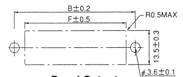
Panel Cutout
