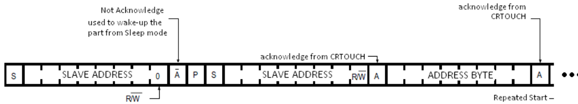
Figure 13. CRTCouch wakeup using I2C communication
