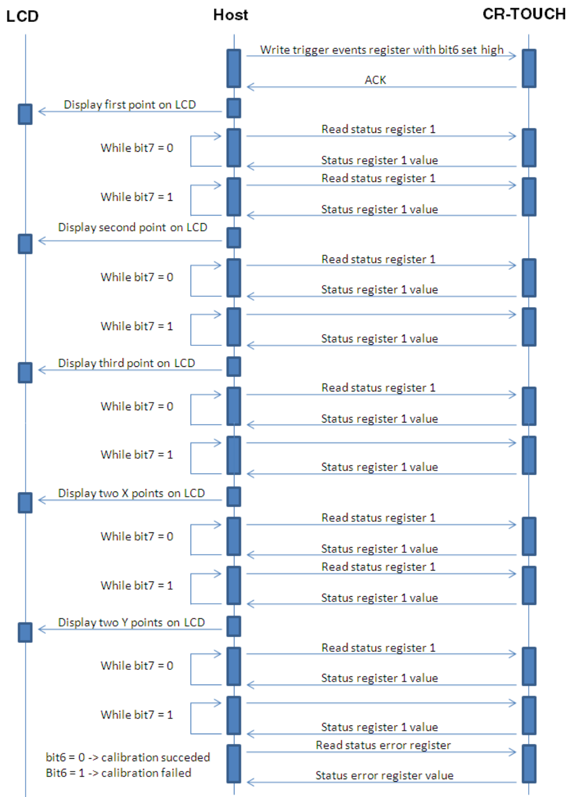
Figure 10. Single and two touch calibration sequence
