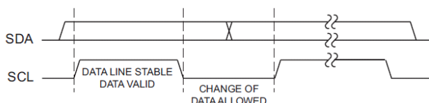
Figure 17. Bit Transfer
