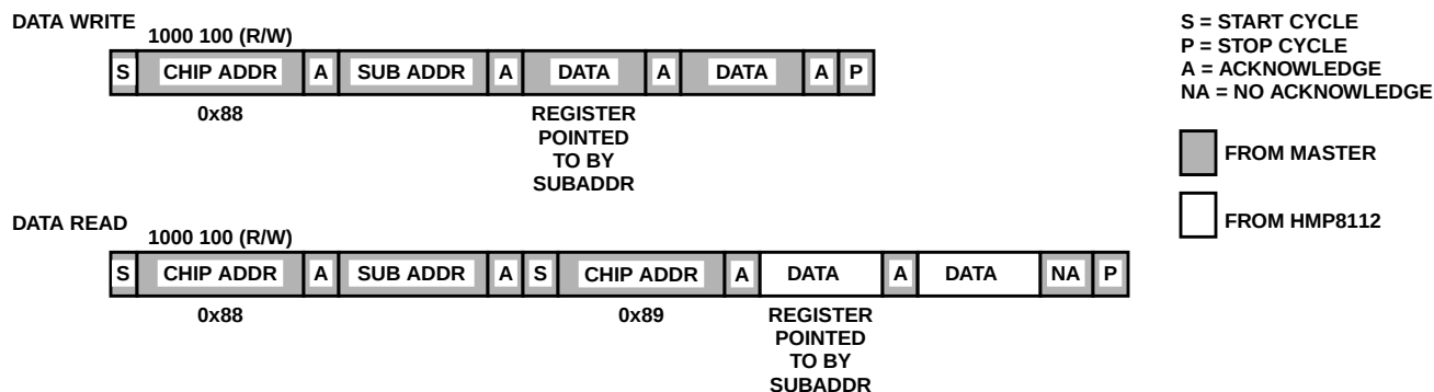
FIGURE 14. REGISTER WRITE PROGRAMMING FLOW
