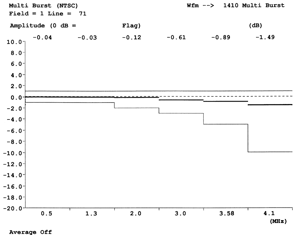
FIGURE 22. MULTIBURST VM700 FREQUENCY ROLL-OFF TEST
