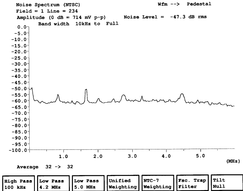
FIGURE 23. SIGNAL TO NOISE RATIO - FLAT FREQUENCY RESPONSE
