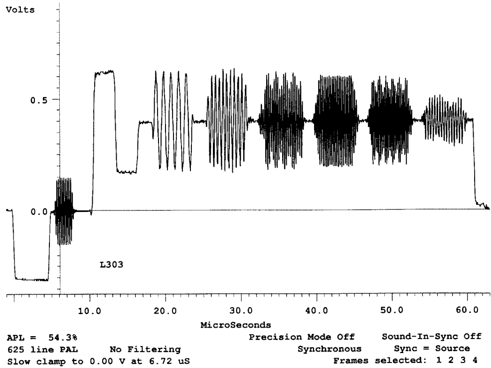
FIGURE 31. MULTIBURST
