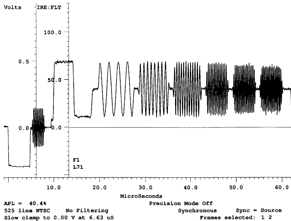
FIGURE 21. MULTIBURST
