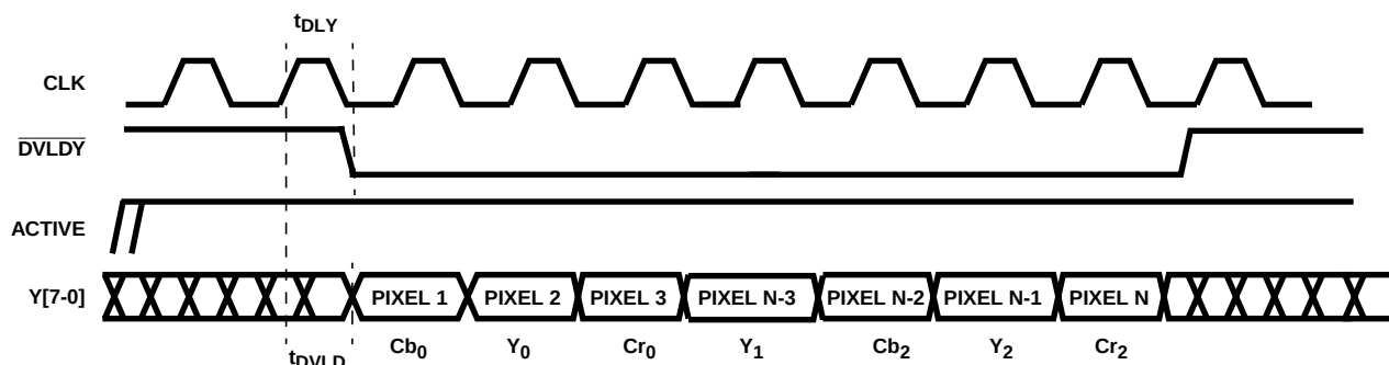
FIGURE 16. OUTPUT TIMING 8-BIT MODE
