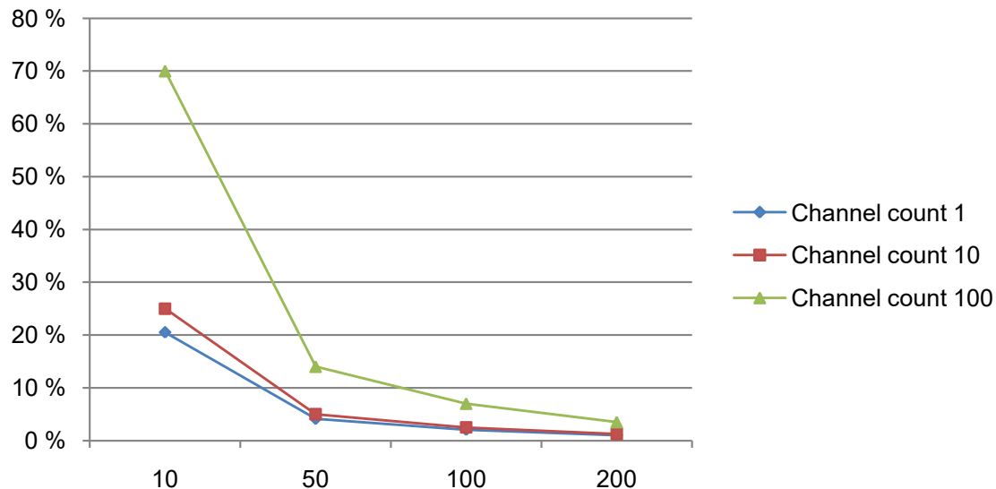
Figure 41-13. CPU Utilization
