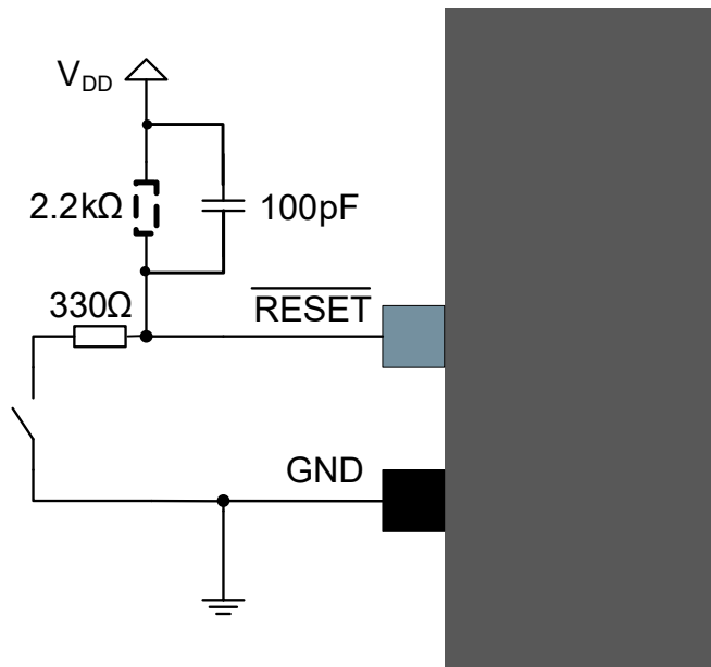
Figure 44-5. External Reset Circuit Schematic (EFT Immunity Enhancement)
