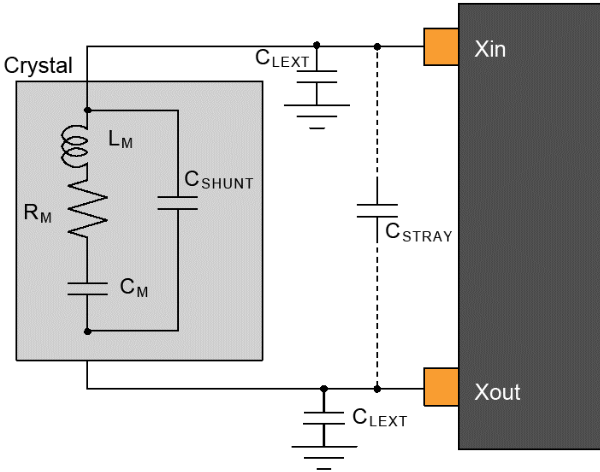
Figure 40-2. Oscillator Connection
