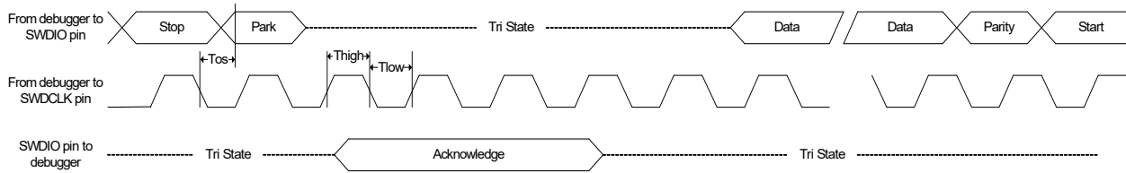
Figure 41-23. SWD Interface Signals
