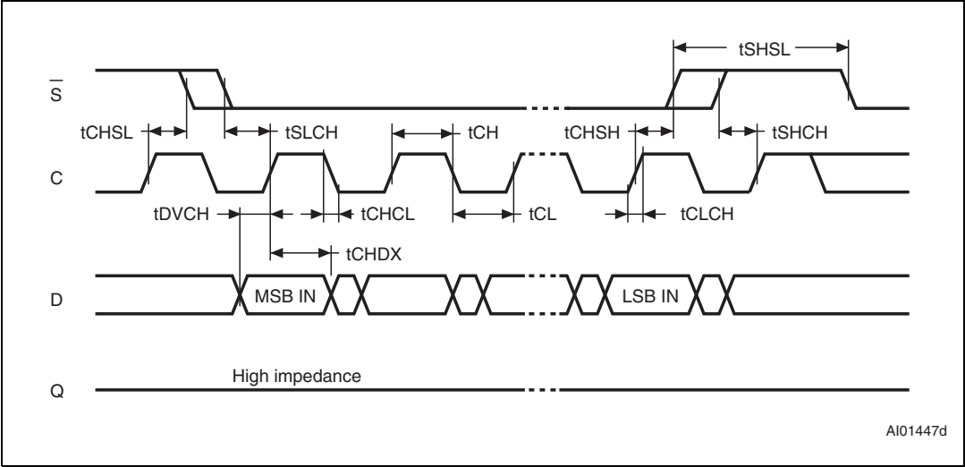
Figure 16. Serial input timing
