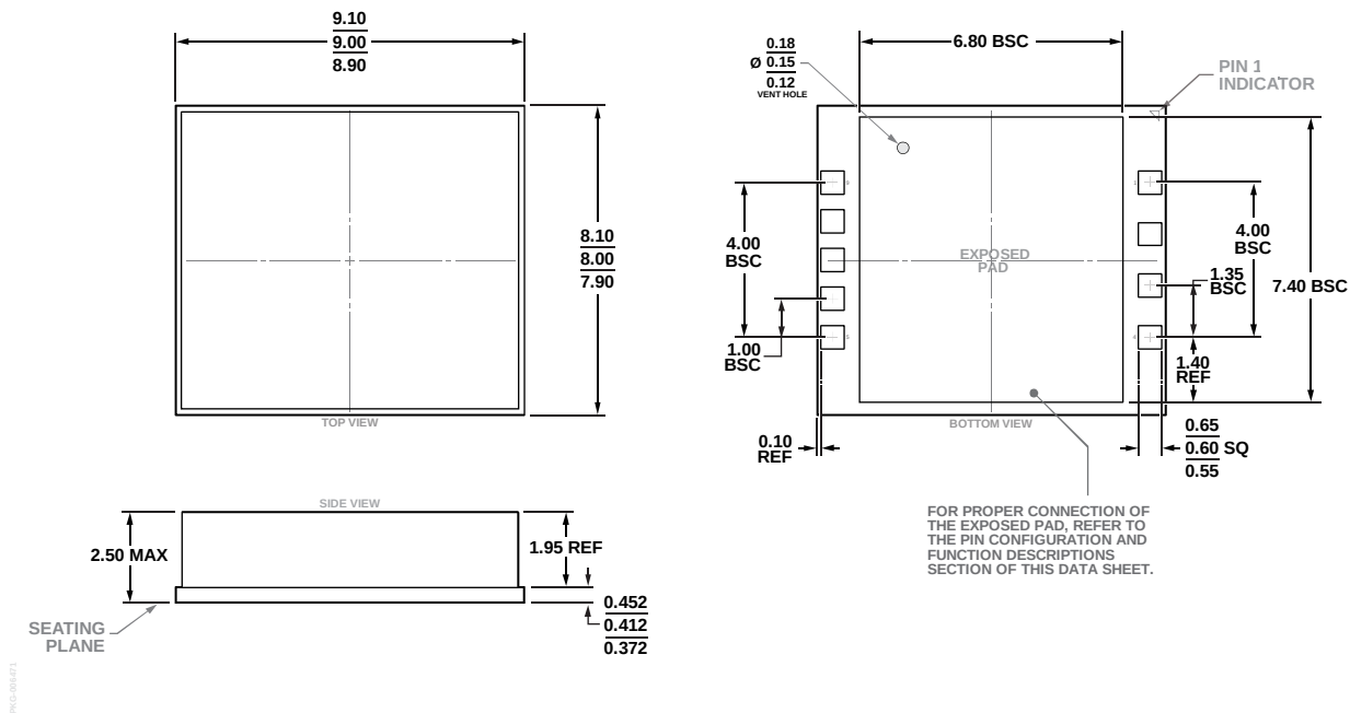
Figure 26. 9-Terminal Chip Array Small Outline No Lead Cavity [LGA_CAV] 9.00 mm × 8.00 mm Body and 2.50 mm Package Height (CE-9-2) Dimensions shown in millimeters
