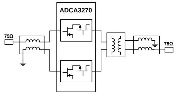
Figure 15. Simplified Schematic
