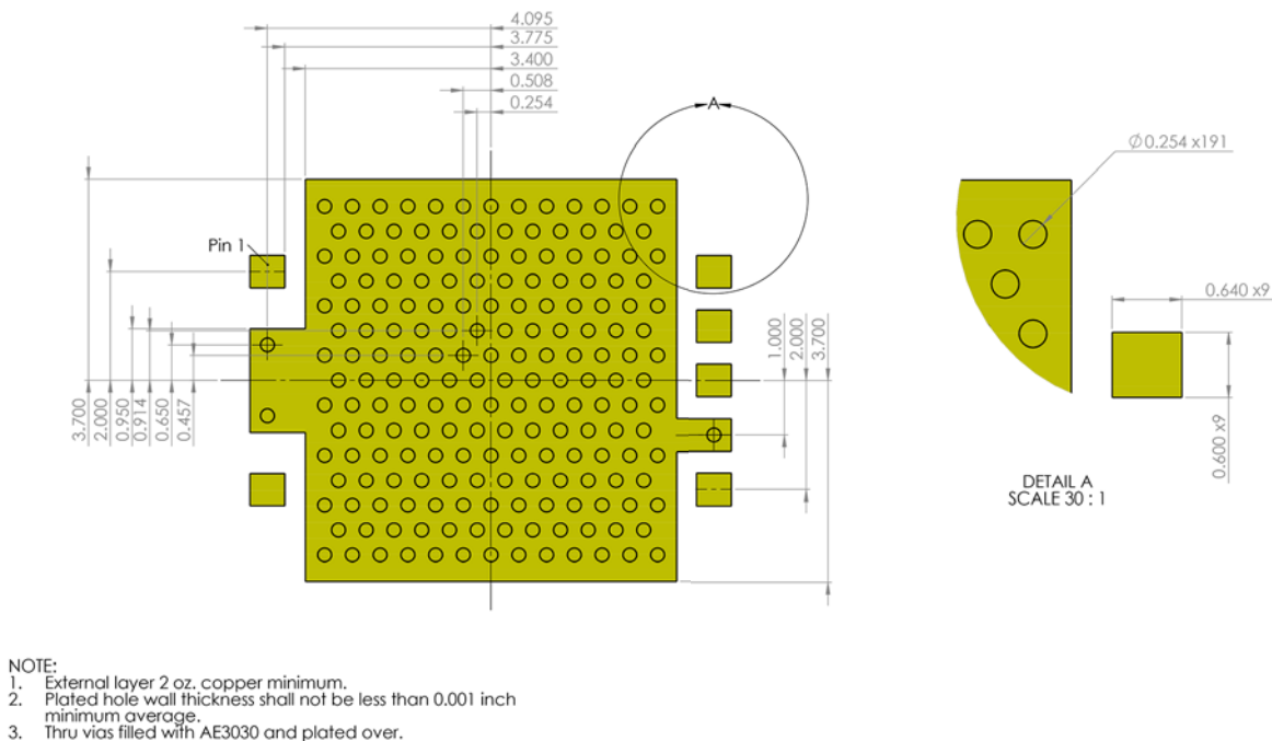
Figure 19. Recommended PCB Layout (Dimensions Shown in Millimeters)
