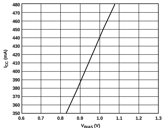
Figure 21. I_{CC} vs. V_{BIAS}
