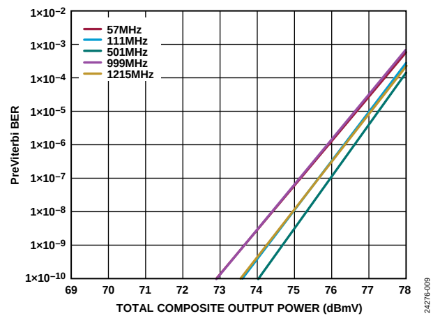
Figure 9. PreViterbi BER vs. Total Composite Output Power at Various Frequencies, 35°C, 9 dB Tilt
