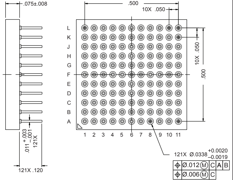
Bottom View
