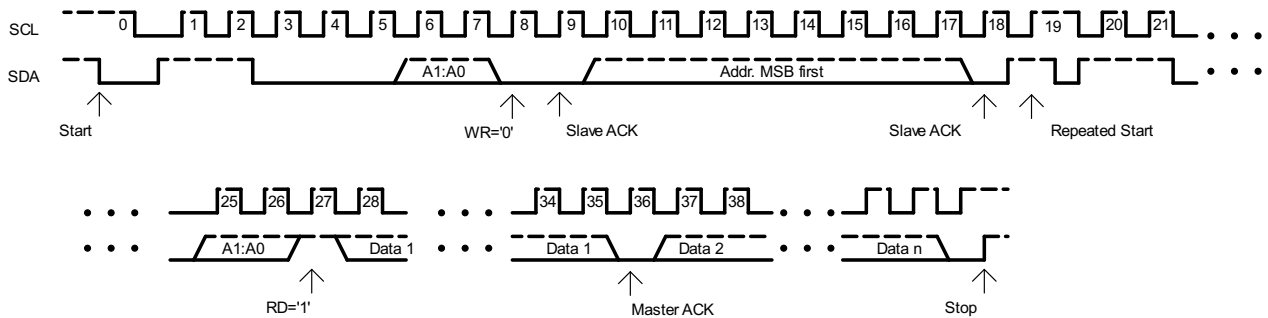
Figure 14: I 2 C read and write commands
