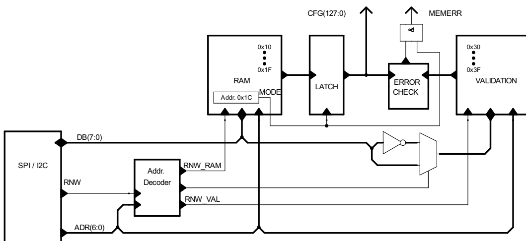
Figure 21: Interface, RAM integrity monitoring and configuration latching
