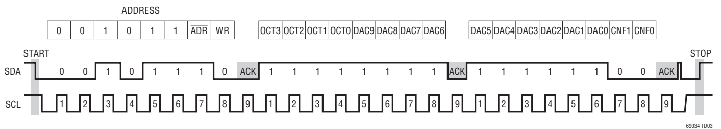
LTC6904 Typical Input Waveform— Programming Frequency to 68MHz (ADR Pin Set LOW)
