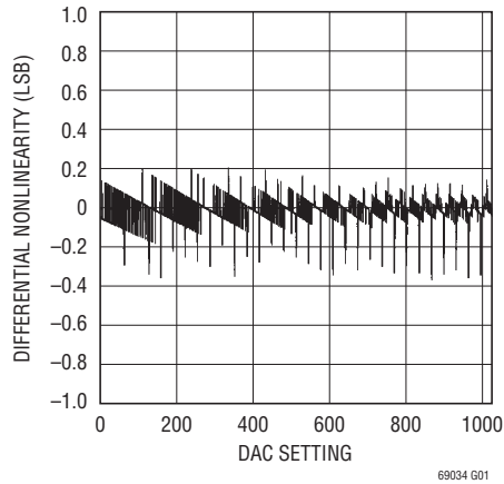
Differential Nonlinearity
