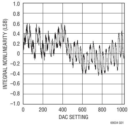
Integral Nonlinearity
