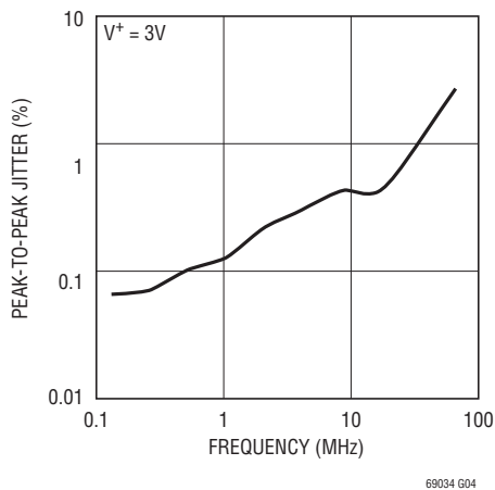
Peak-to-Peak Jitter vs Frequency
