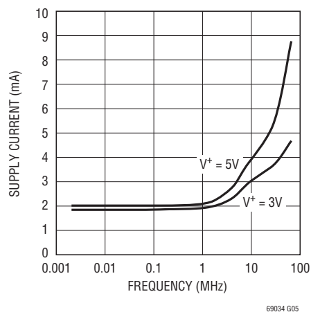
Supply Current vs Output Frequency
