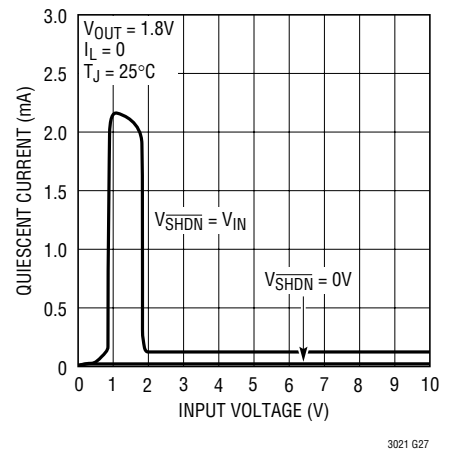
Quiescent Current
