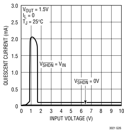
Quiescent Current
