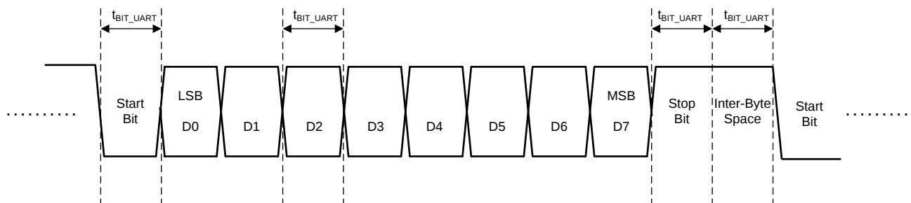
图 20. USART Asynchronous Interface Bit Timing
