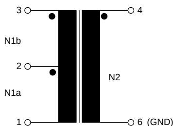
图 138. Typical Pinout of Center-Tap Transformer for Ultrasonic Transducers
