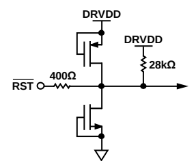
Figure 41. Equivalent \overline{RST} Input Circuit
