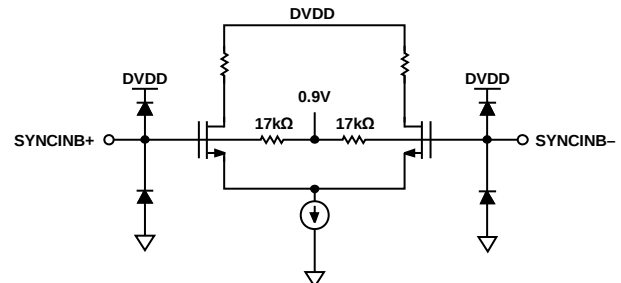
Figure 39. Equivalent SYNCINB± Input Circuit
