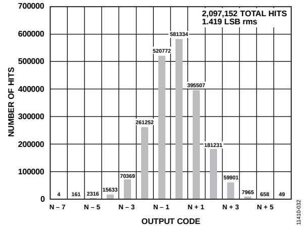
Figure 32. AD9683-250 Grounded Input Histogram
