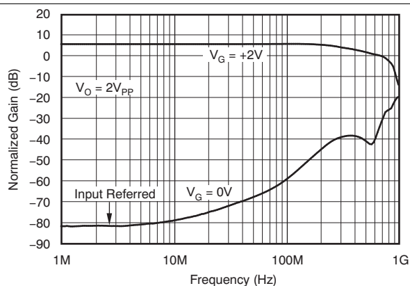
Figure 25. Fully-Attenuated Response
