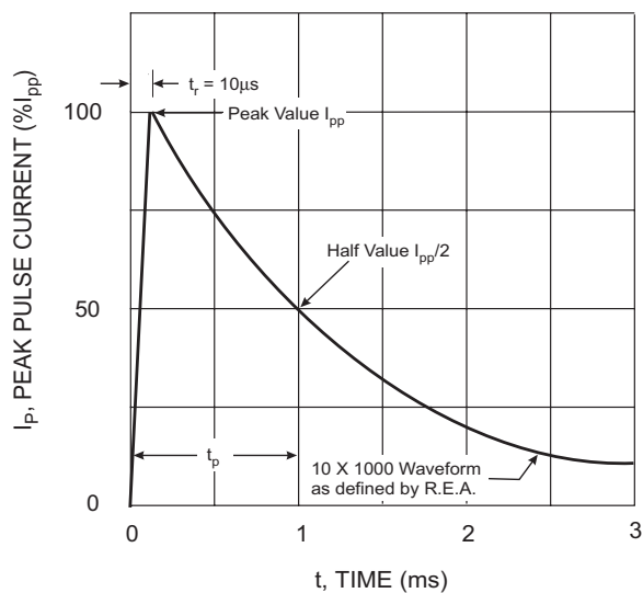
Fig. 4 Pulse Waveform
