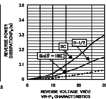
VR-P 2 CHARACTERISTICS
