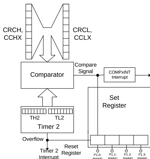
FIGURE 24: TIMER 2 COMPARE MODE 0 BLOCK DIAGRAM
