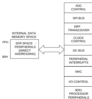
FIGURE 8: SFR ORGANIZATION
