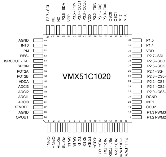
FIGURE 3: VMX51C1020 PINOUT
