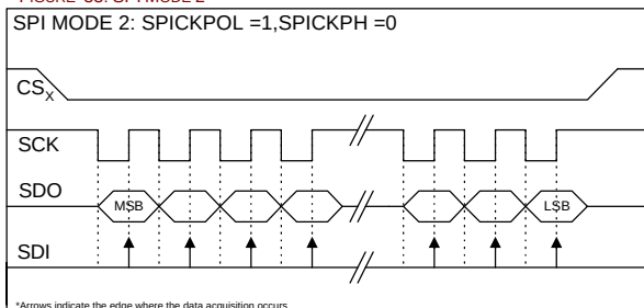
FIGURE 33: SPI MODE 2
