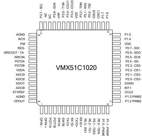
FIGURE 2: VMX51C1020 QFP-64 PACKAGE PINOUT
