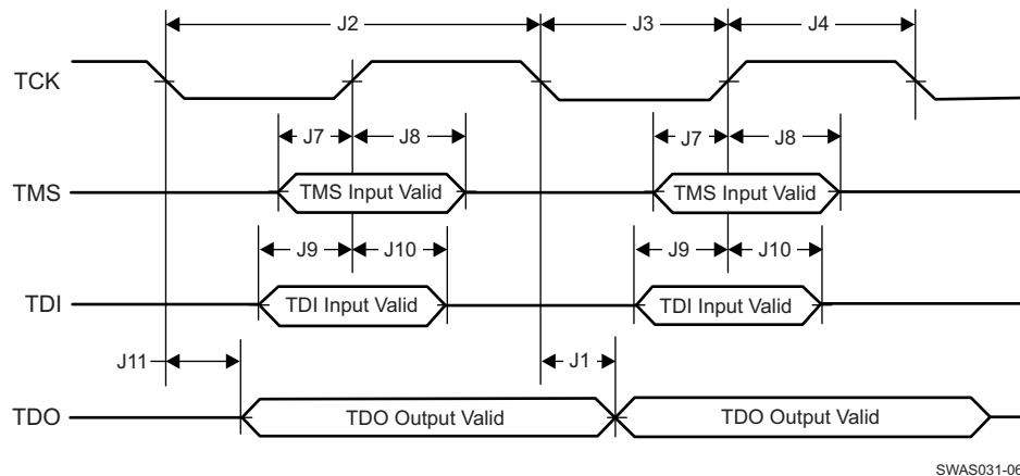
Figure 4-15. JTAG Timing
