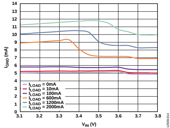
Figure 14. Ground Current ( I_{GND} ) vs. Input Voltage ( V_{IN} ) in Dropout, V_{OUT} = 3.3\text{ V}
