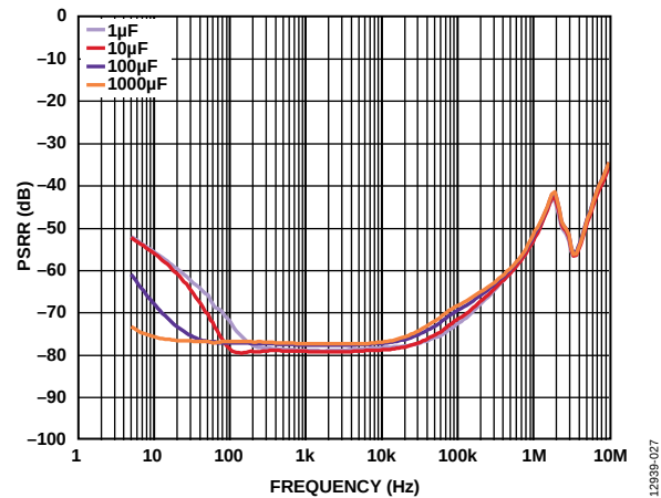
Figure 27. Power Supply Rejection Ratio (PSRR) vs. Frequency at Various C_{BYF} Values, V_{OUT} = 3.3\text{ V} , V_{IN} = 4.0\text{ V} , 2 A Load
