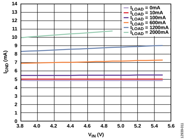
Figure 11. Ground Current ( I_{GND} ) vs. Input Voltage ( V_{IN} ) at Various Loads, V_{OUT} = 3.3\text{ V}
