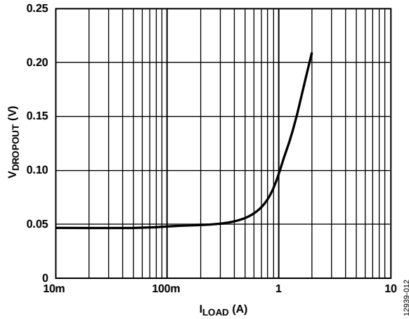
Figure 12. Dropout Voltage ( V_{DROP} ) vs. Load Current ( I_{LOAD} ), V_{OUT} = 3.3\text{ V}
