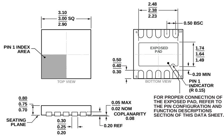
Figure 65. 10-Lead Lead Frame Chip Scale Package [LFCSP] 3 mm × 3 mm Body and 0.75 mm Package Height (CP-10-9)
