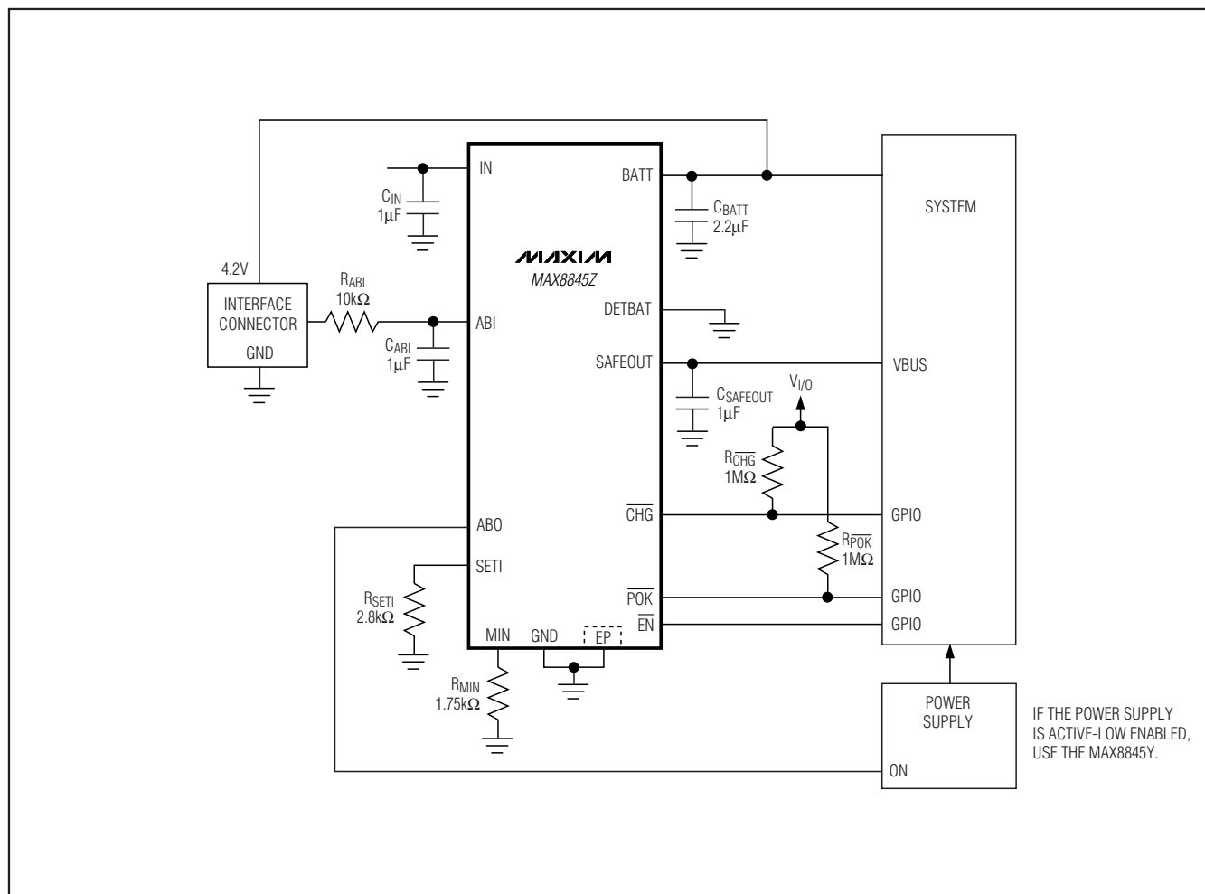
Figure 4. Factory System Interface Connector Application
