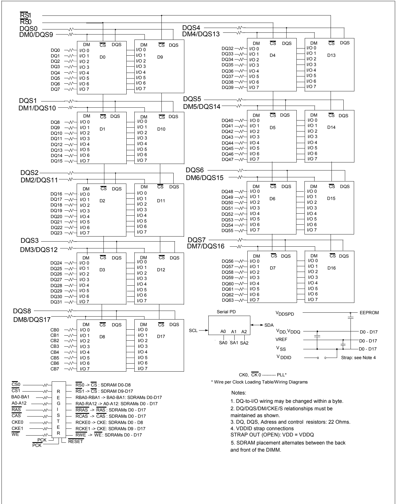
Figure 3 Block Diagram: Two Ranks 64M × 72 DDR-I SDRAM DIMM Module (32M×8 components) HYS 72D64320GBR on Raw Card B
