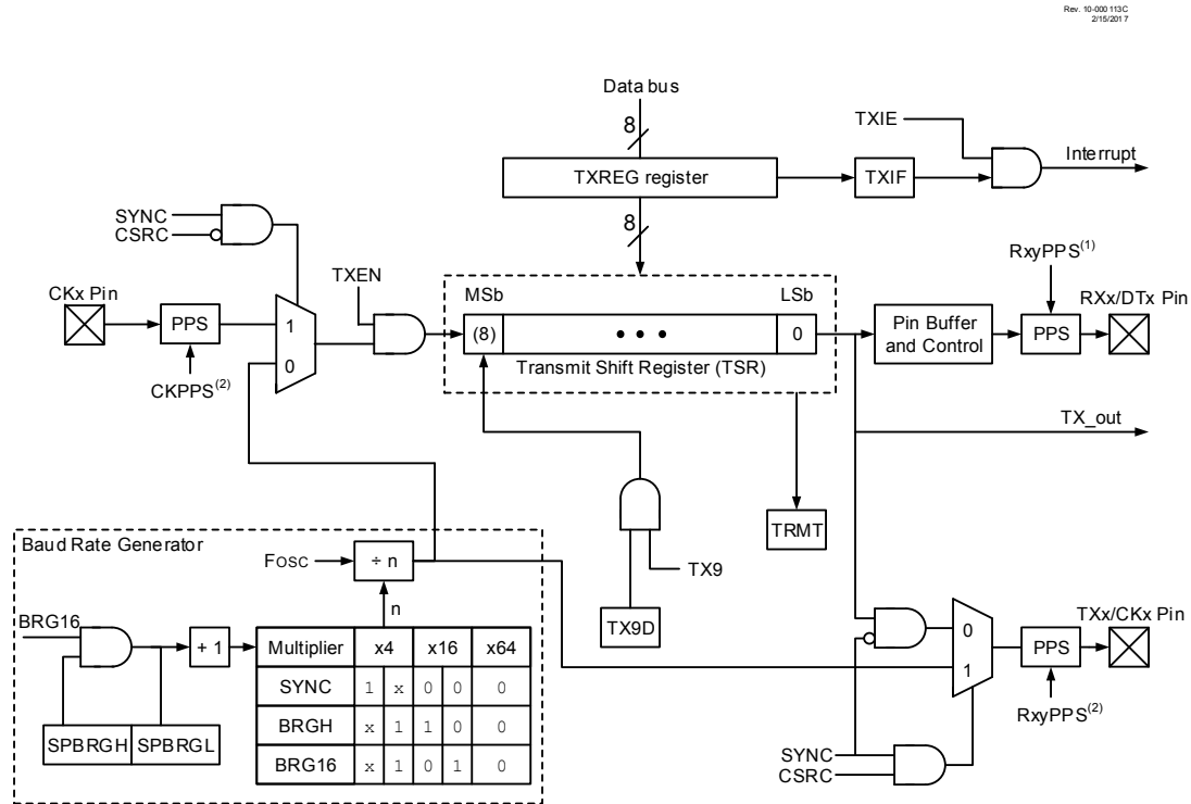
Figure 29-1. EUSART Transmit Block Diagram
