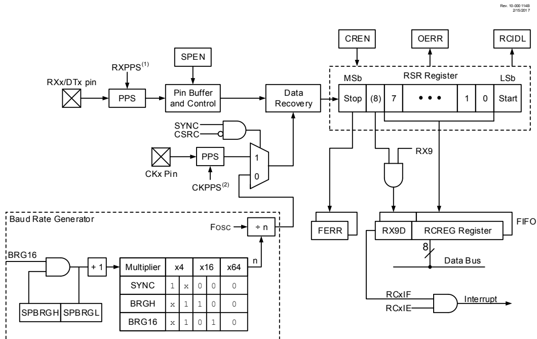
Figure 29-2. EUSART Receive Block Diagram
