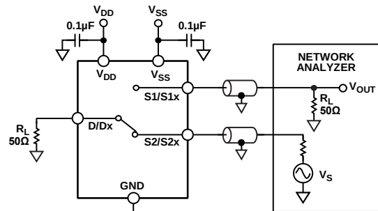
Figure 41. Bandwidth
