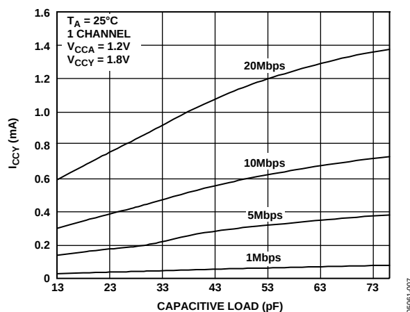
Figure 7. I_{CCY} vs. Capacitive Load at Pin Y for A Y (1.2 V 1.8 V) Level Translation
