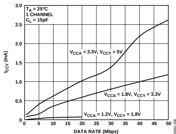
Figure 6. I_{CCY} vs. Data Rate (Y A Level Translation)
