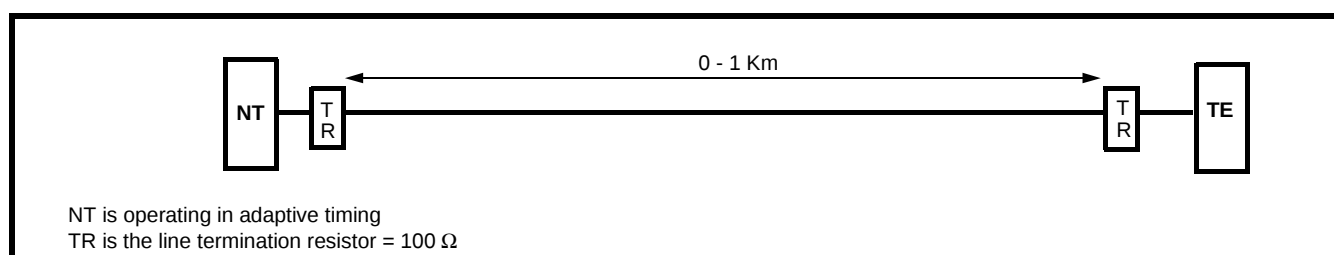
Figure 8 - Point-to-Point Configuration
