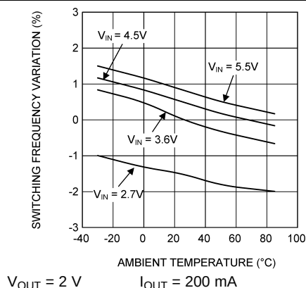
Figure 5. Switching Frequency vs Temperature
