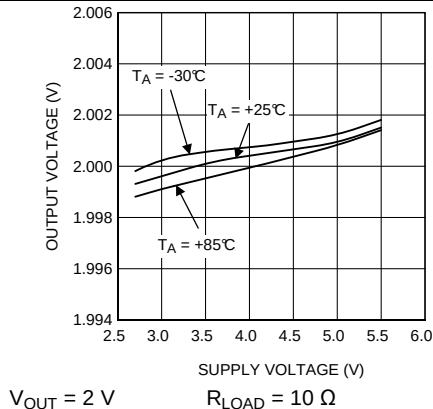
Figure 6. Output Voltage vs Supply Voltage
