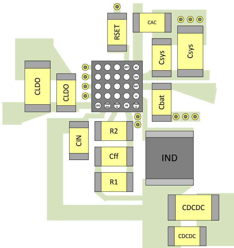
Figure 41. Layout Recommendation
