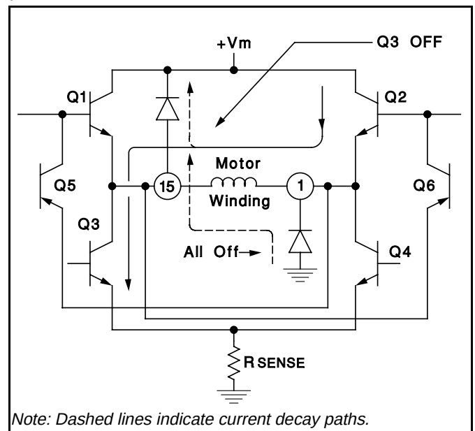
Figure 7. Simplified Schematic of Output Stage
