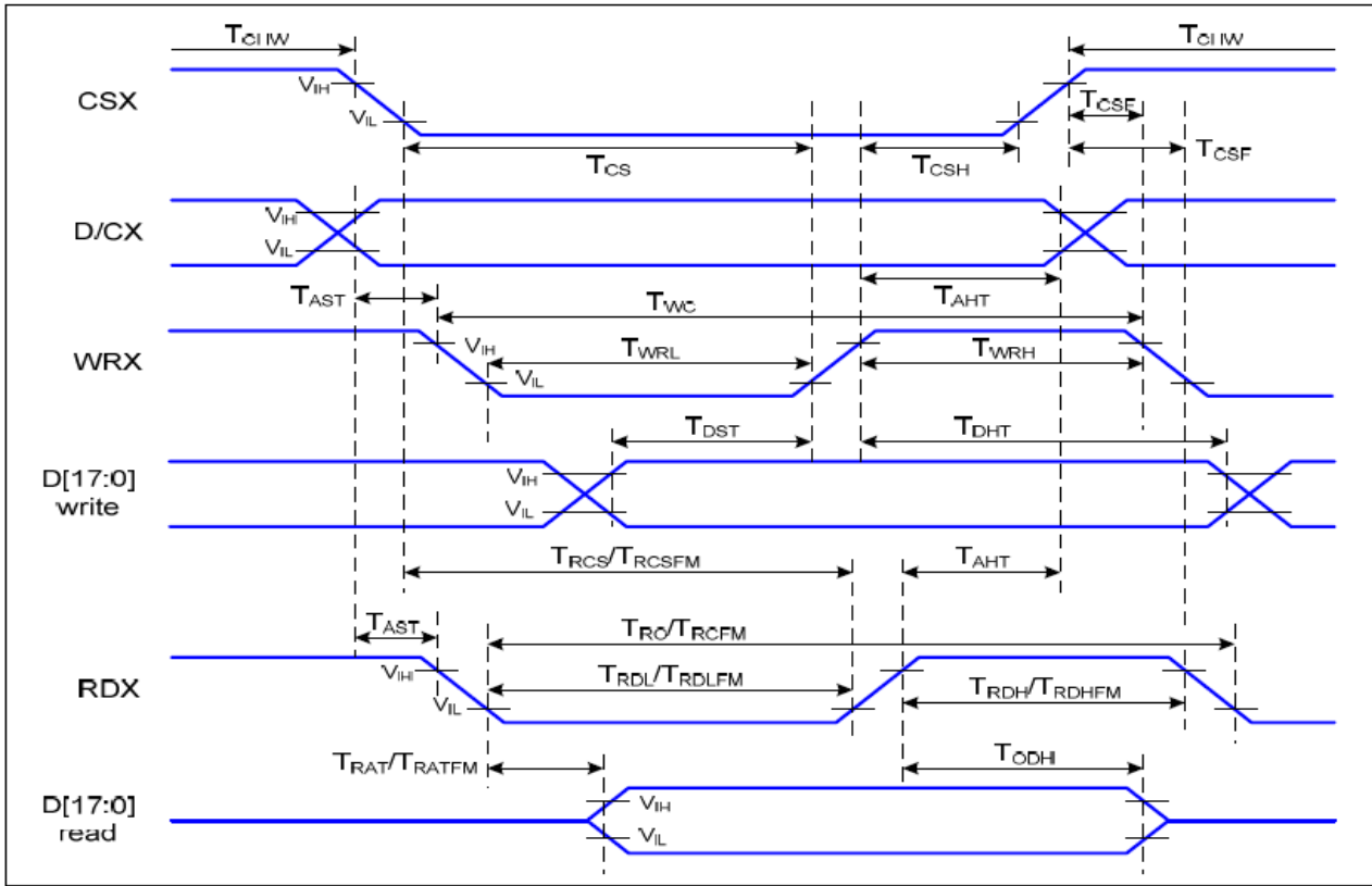
Figure 1 Parallel Interface Timing Characteristics (8080 Series MCU Interface)
