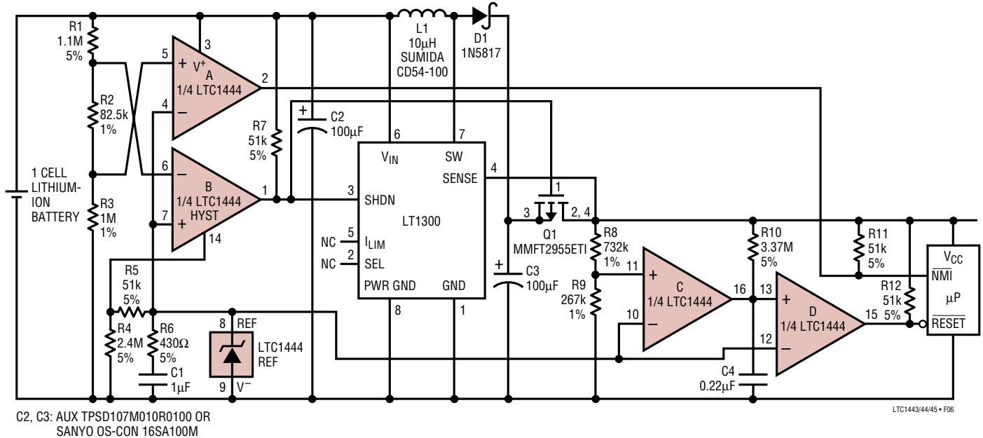
Single Cell to 5V Supply
