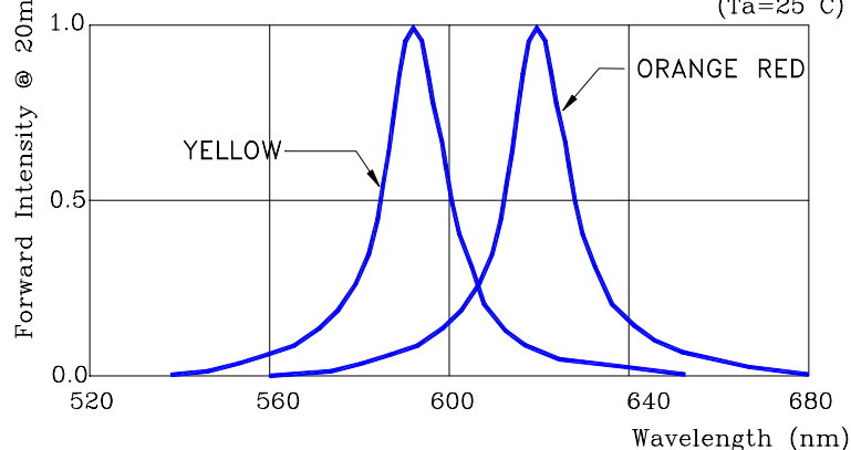
FIG. 5 Relative Intensity vs. Wavelength ( λ p) (Ta=25 °C)
