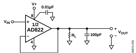
Figure 35. Unity-Gain Follower
