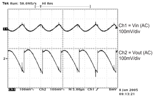
Ripple 200mA Torch, Vin = 3.6V, Vout = 3.9V
