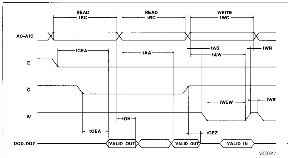
Figure 3. Read-Read-Write Timing
