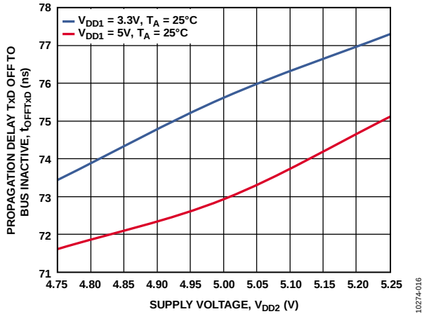
Figure 9. Propagation Delay from TxD Off to Bus Inactive vs. Supply Voltage, V_{DD2}
