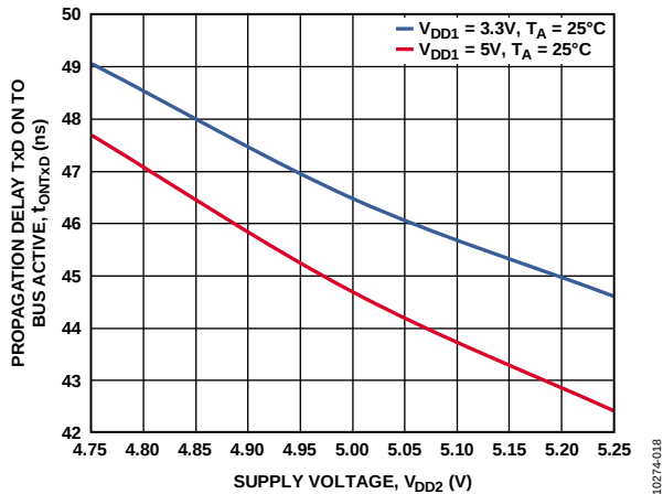
Figure 11. Propagation Delay from TxD On to Bus Active vs. Supply Voltage, V_{DD2}
