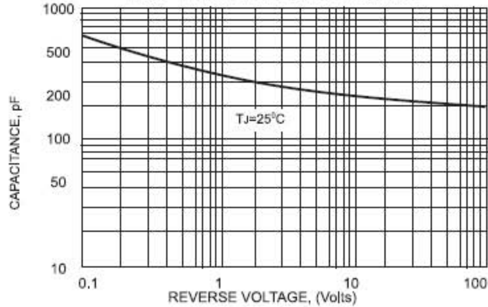
FIG.5 - TYPICAL JUNCTION CAPACITANCE
