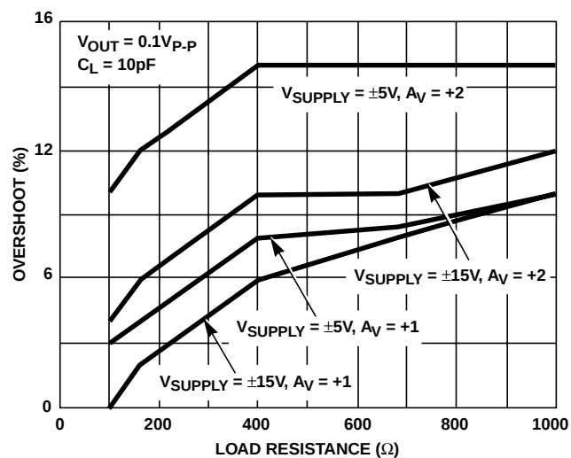
FIGURE 18. SMALL SIGNAL OVERSHOOT vs LOAD RESISTANCE
