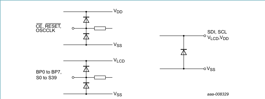
Fig 36. Device protection diagram for PCF8545B
