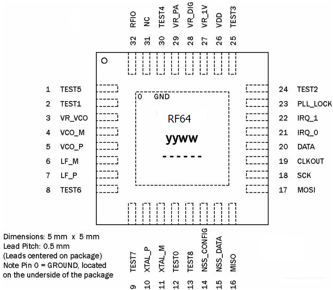
Figure 2: RF64 Pin Diagram
