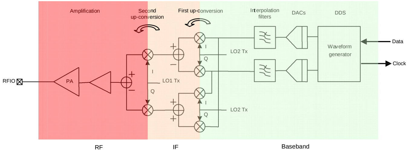
Figure 8: Transmitter Architecture
