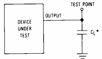
Figure 2. Test Circuit
