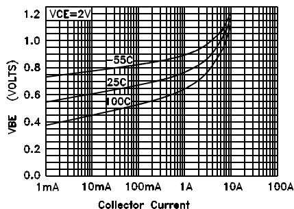
FIG. 5 V_{BE(ON)} vs I_C
