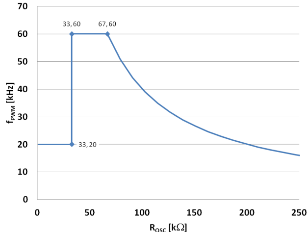
Figure 4. PWM Clock Frequency Setting
