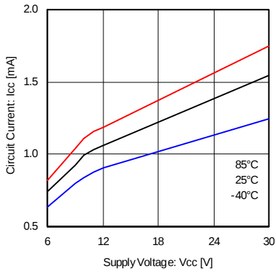
Fig.3 Supply current
