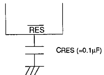
Fig. 4 Reset Circuit
