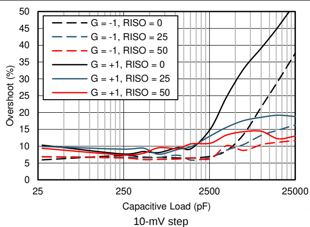
Figure 28. Small-Signal Overshoot vs Capacitive Load
