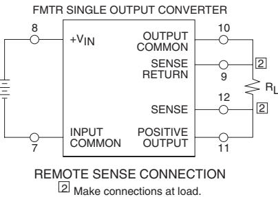
FIGURE 3: REMOTE SENSE 2, 3
