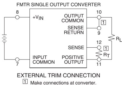
FIGURE 2: TRIM CONNECTION 1, 2, 3
