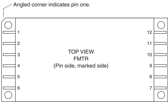
FIGURE 4: PIN OUT
